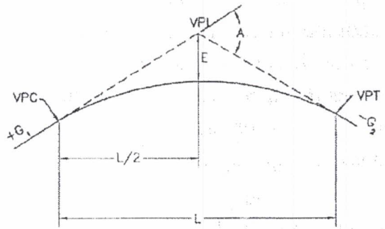
Figure 5: Summit Curve
