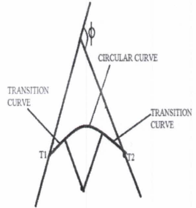
Figure 12: Transition Curve
